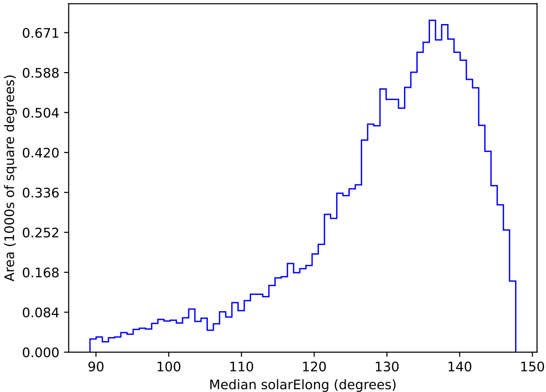
too_10_4v3.4_10yrs WFD r band: Median solarElong
