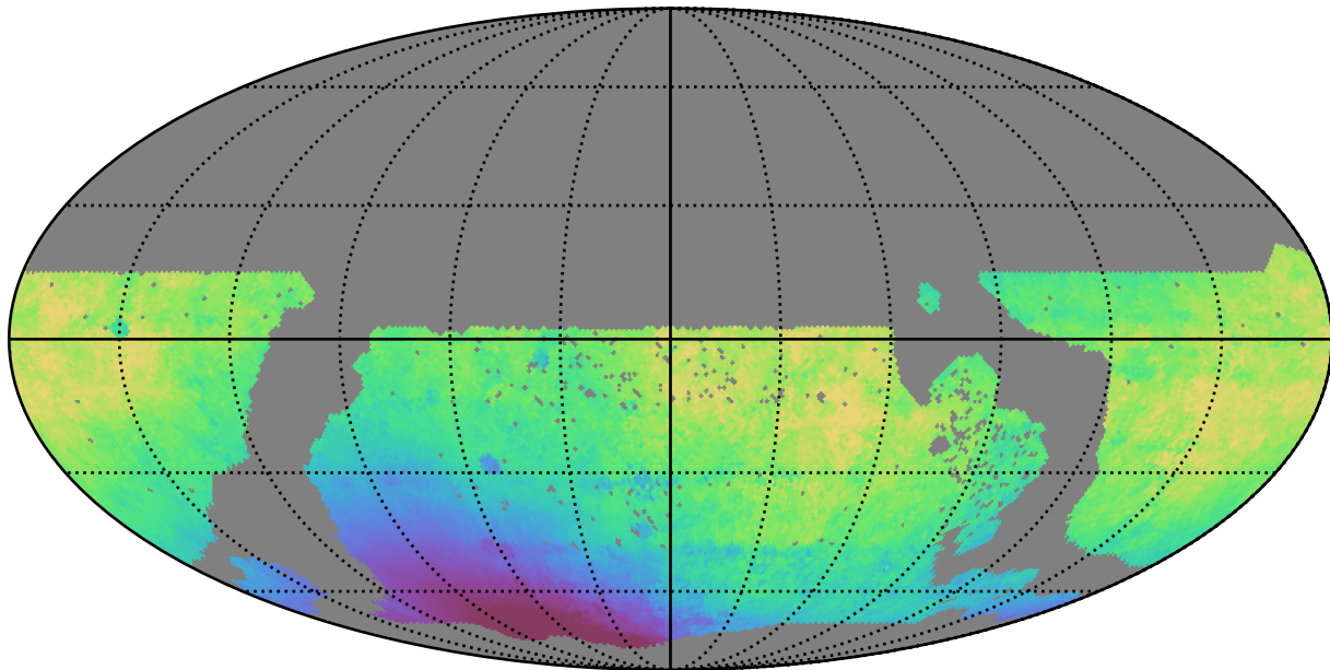
too_10_4v3.4_10yrs WFD i band: Median solarElong
