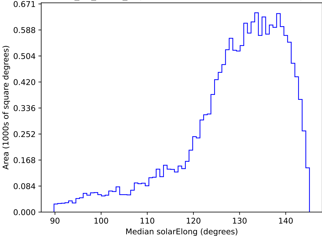
too_10_4v3.4_10yrs WFD i band: Median solarElong
