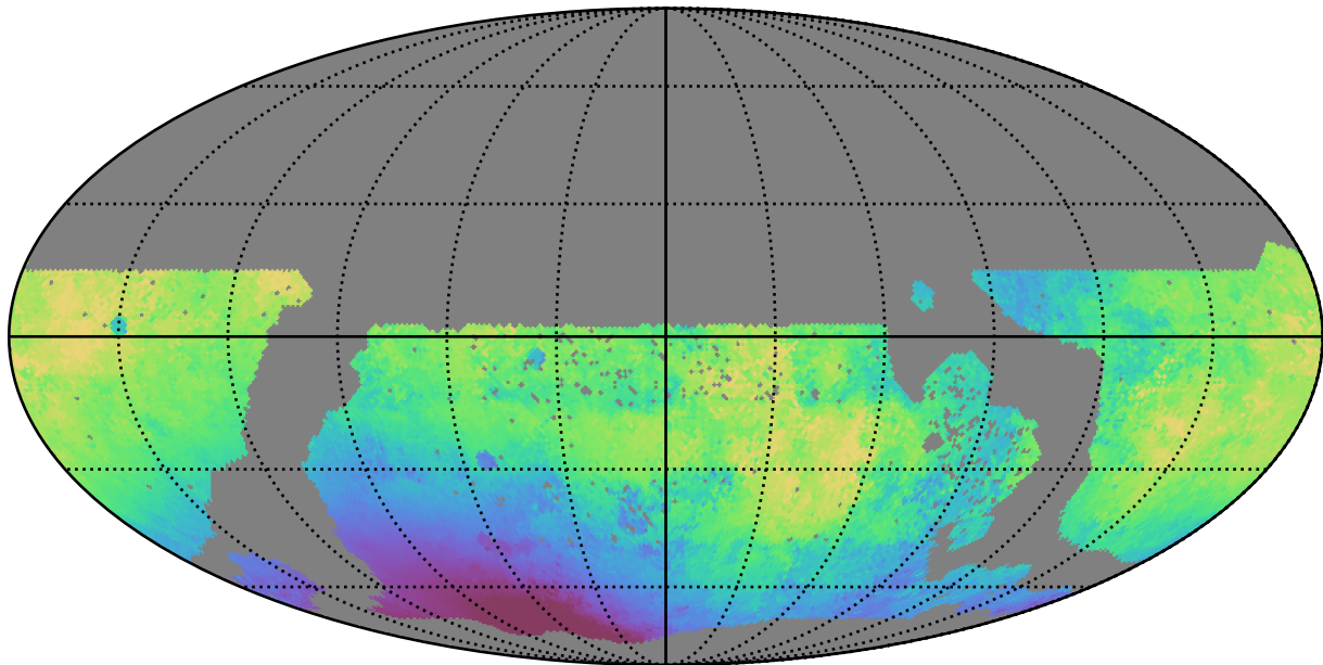
too_10_4v3.4_10yrs WFD g band: Median solarElong
