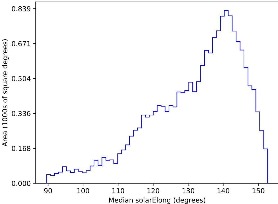
too_10_4v3.4_10yrs WFD g band: Median solarElong
