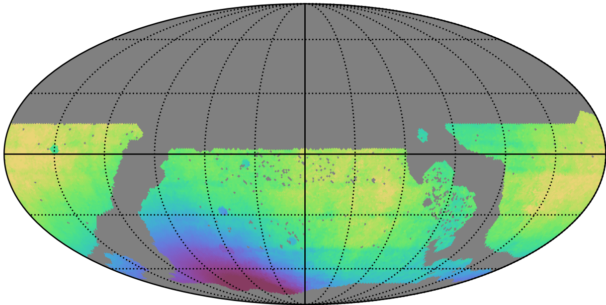
too_10_4v3.4_10yrs WFD all bands: Median solarElong
