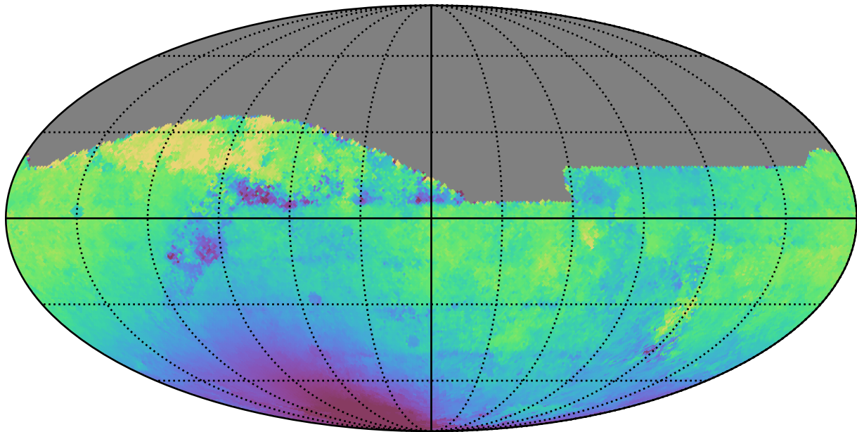
too_10_4v3.4_10yrs All sky z band: Median solarElong
