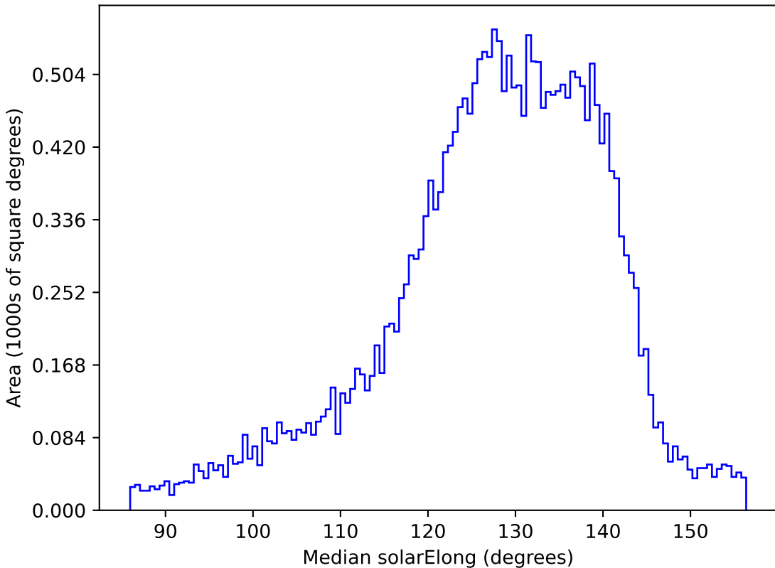
too_10_4v3.4_10yrs All sky z band: Median solarElong
