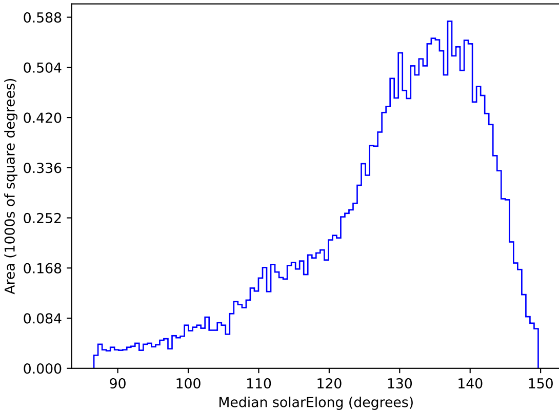
too_10_4v3.4_10yrs All sky y band: Median solarElong
