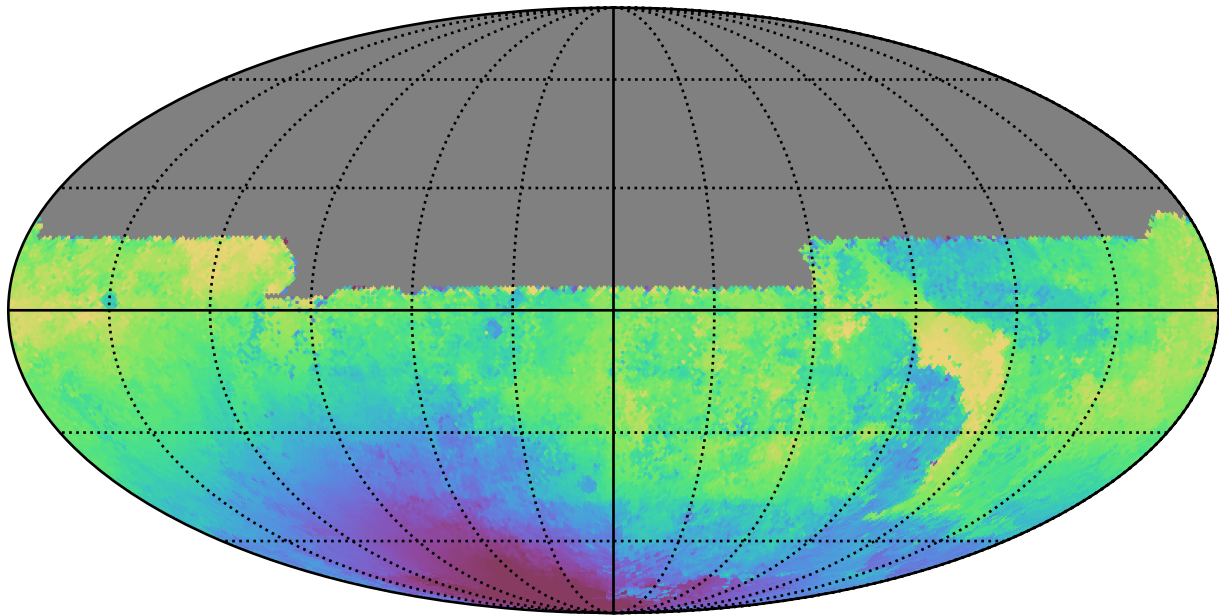
too_10_4v3.4_10yrs All sky u band: Median solarElong
