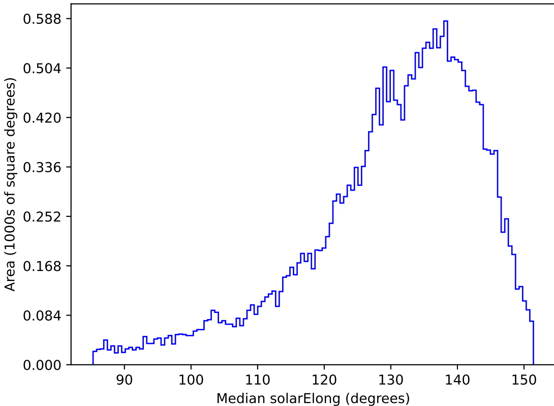
too_10_4v3.4_10yrs All sky r band: Median solarElong
