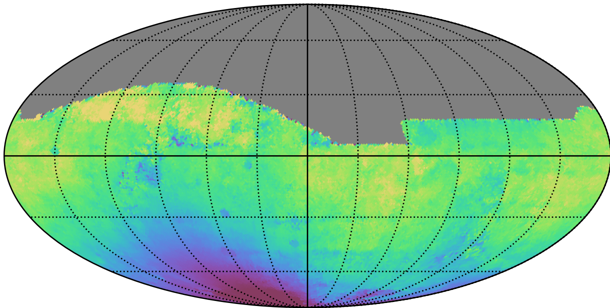
too_10_4v3.4_10yrs All sky i band: Median solarElong
