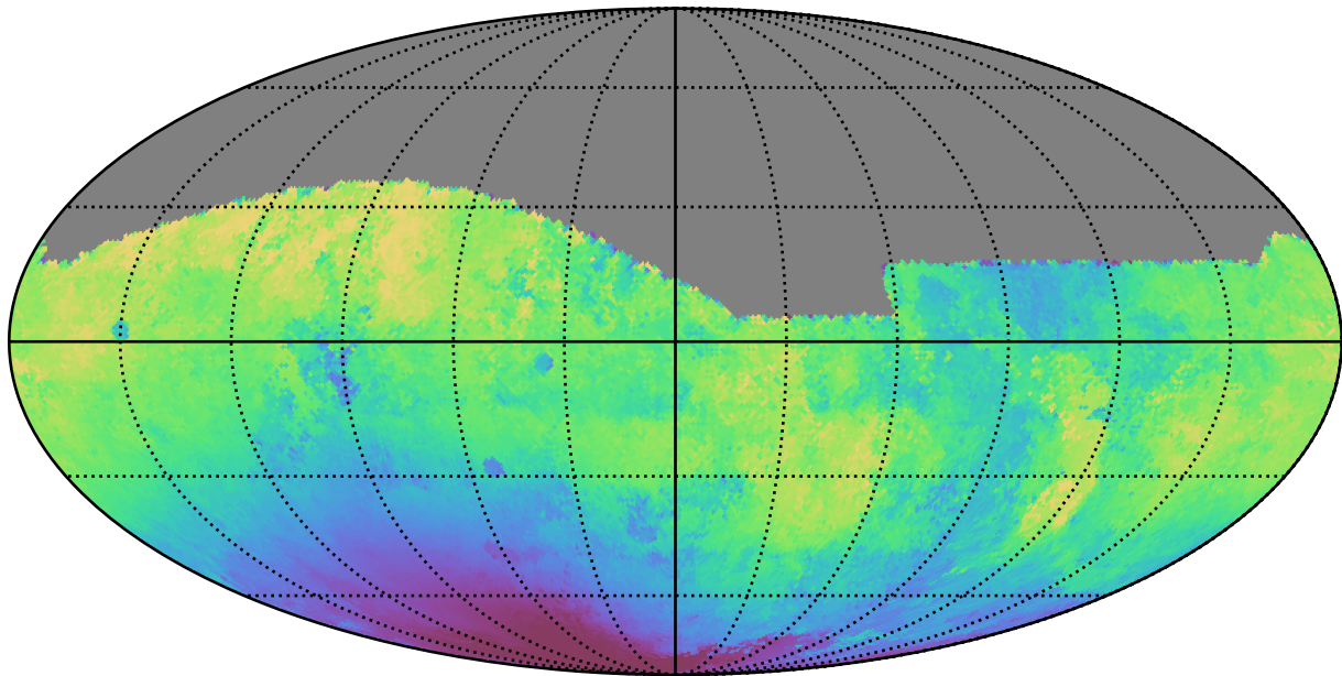
too_10_4v3.4_10yrs All sky g band: Median solarElong
