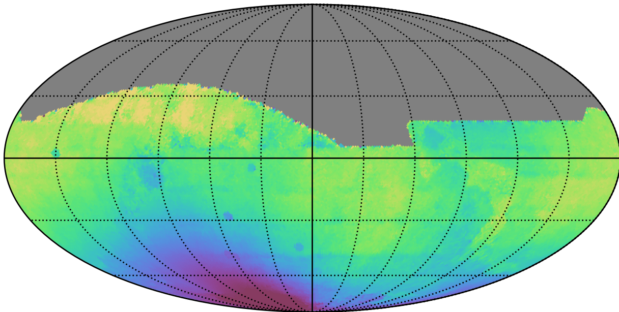
too_10_4v3.4_10yrs All sky all bands: Median solarElong
