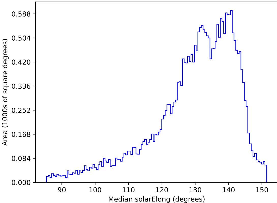
too_10_4v3.4_10yrs All sky all bands: Median solarElong
