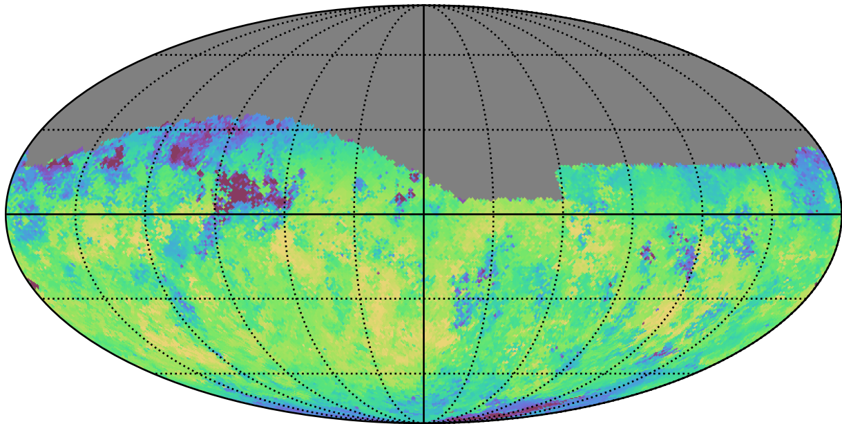
too_10_4v3.4_10yrs Yr 1 z band: Median skyBrightness
