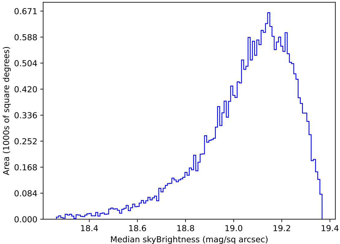
too_10_4v3.4_10yrs Yr 1 z band: Median skyBrightness
