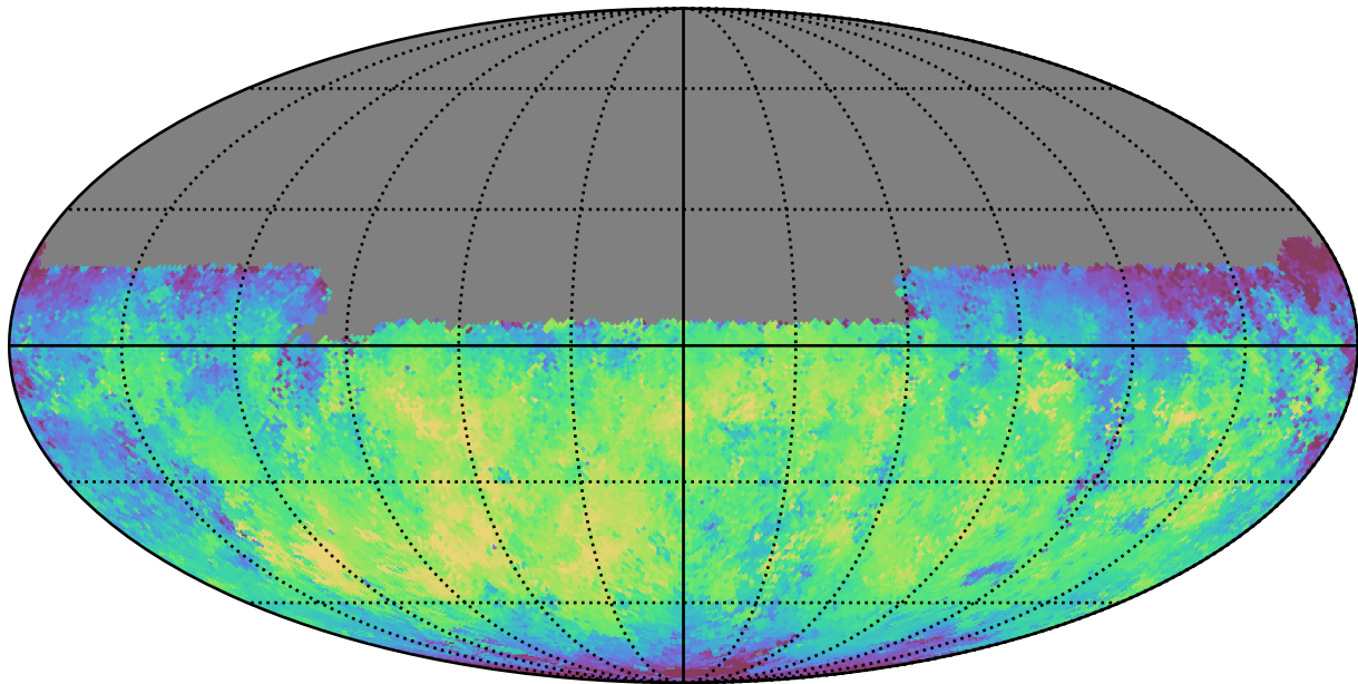
too_10_4v3.4_10yrs Yr 1 y band: Median skyBrightness
