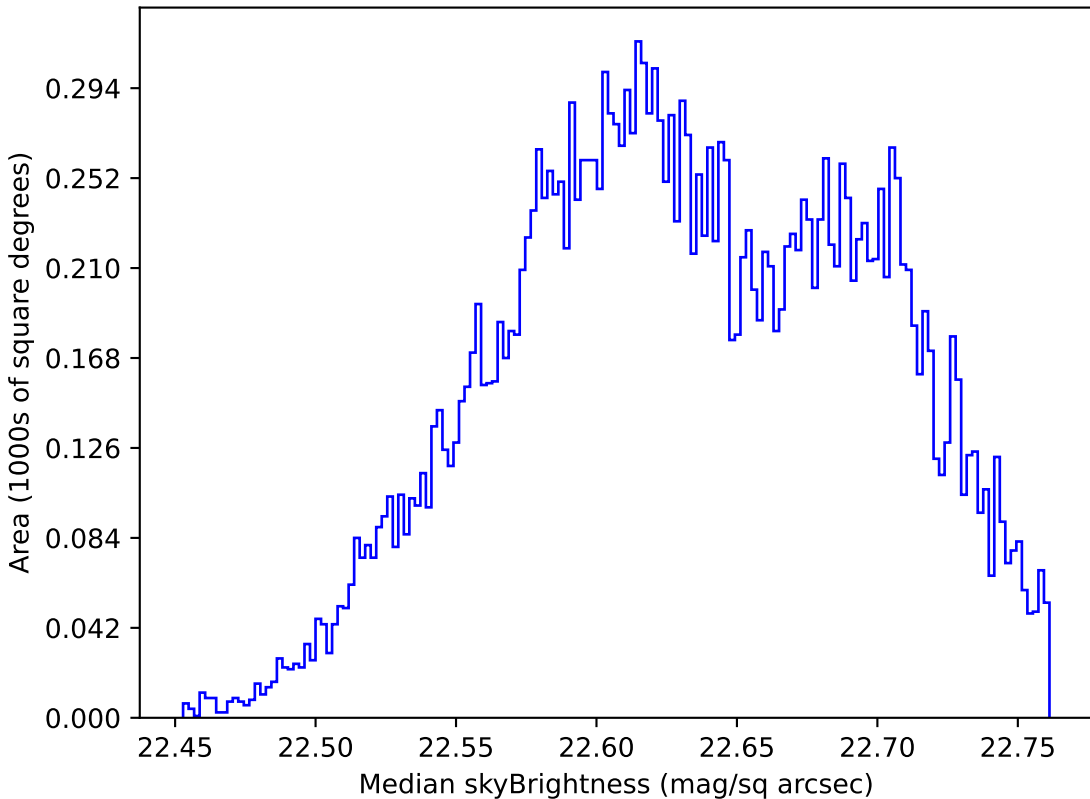
too_10_4v3.4_10yrs Yr 1 u band: Median skyBrightness
