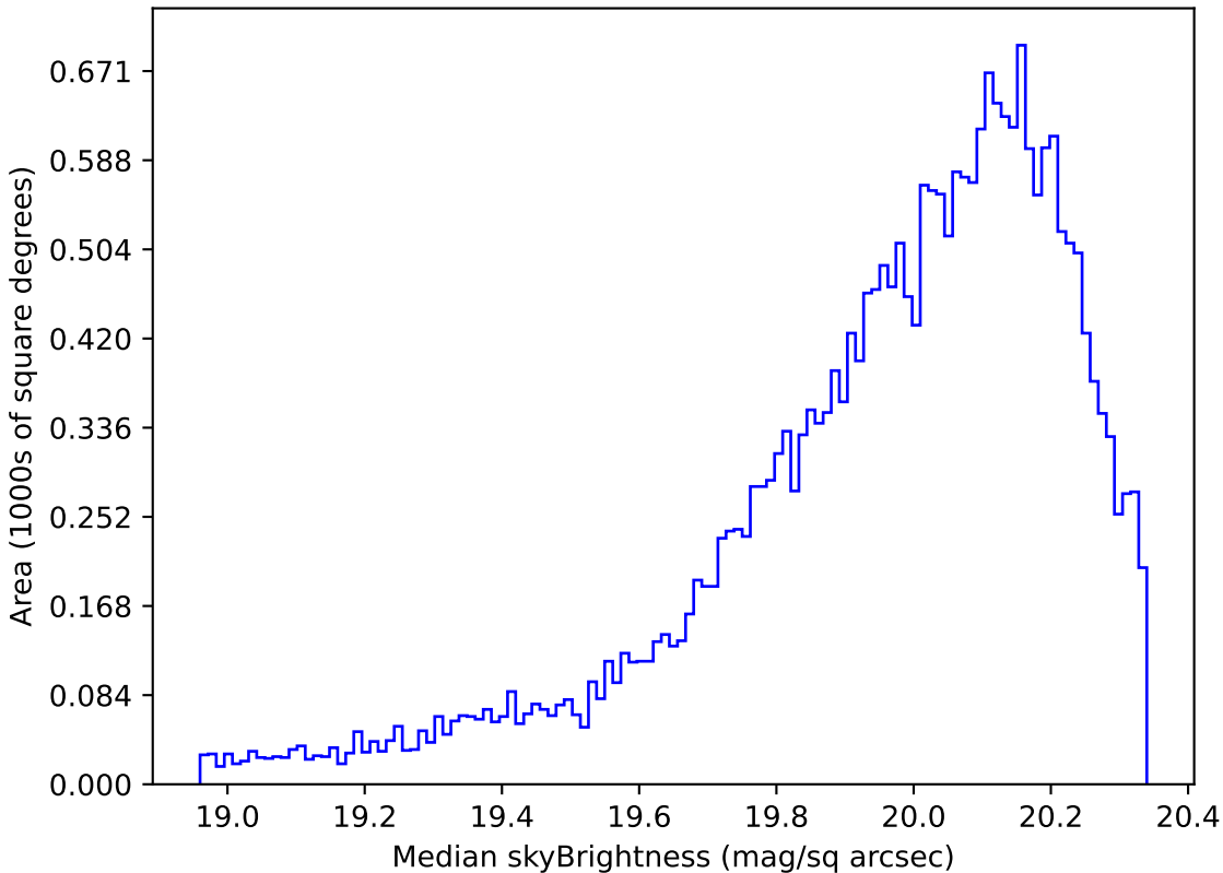
too_10_4v3.4_10yrs Yr 1 i band: Median skyBrightness
