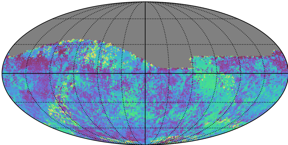
too_10_4v3.4_10yrs Yr 1 all bands: Median skyBrightness
