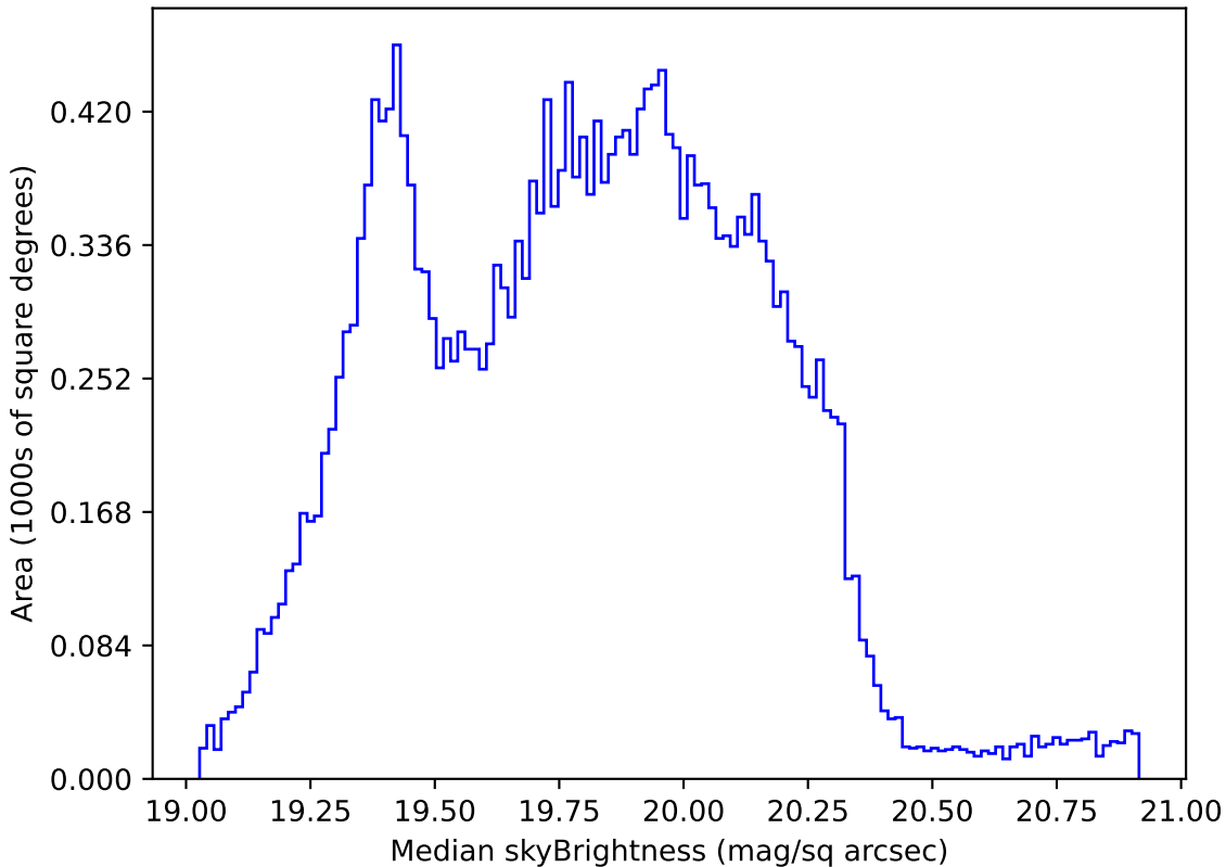
too_10_4v3.4_10yrs Yr 1 all bands: Median skyBrightness
