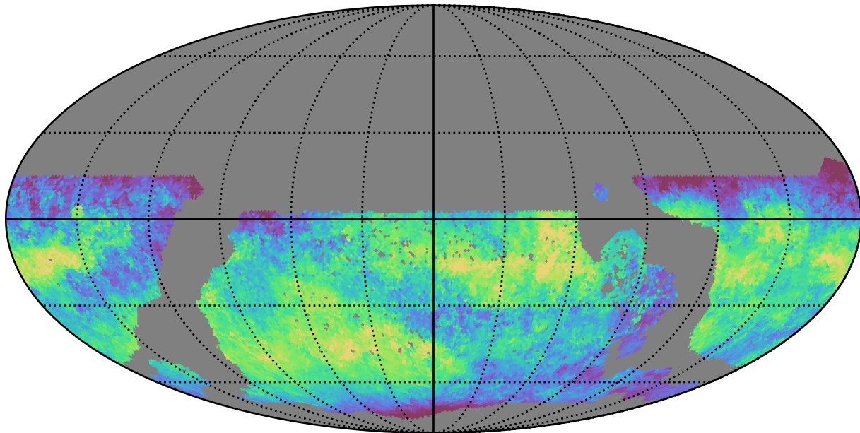
too_10_4v3.4_10yrs WFD z band: Median skyBrightness
