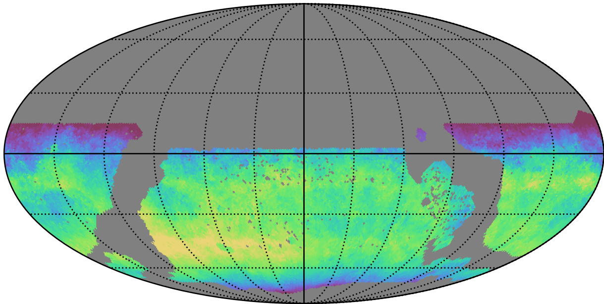
too_10_4v3.4_10yrs WFD y band: Median skyBrightness
