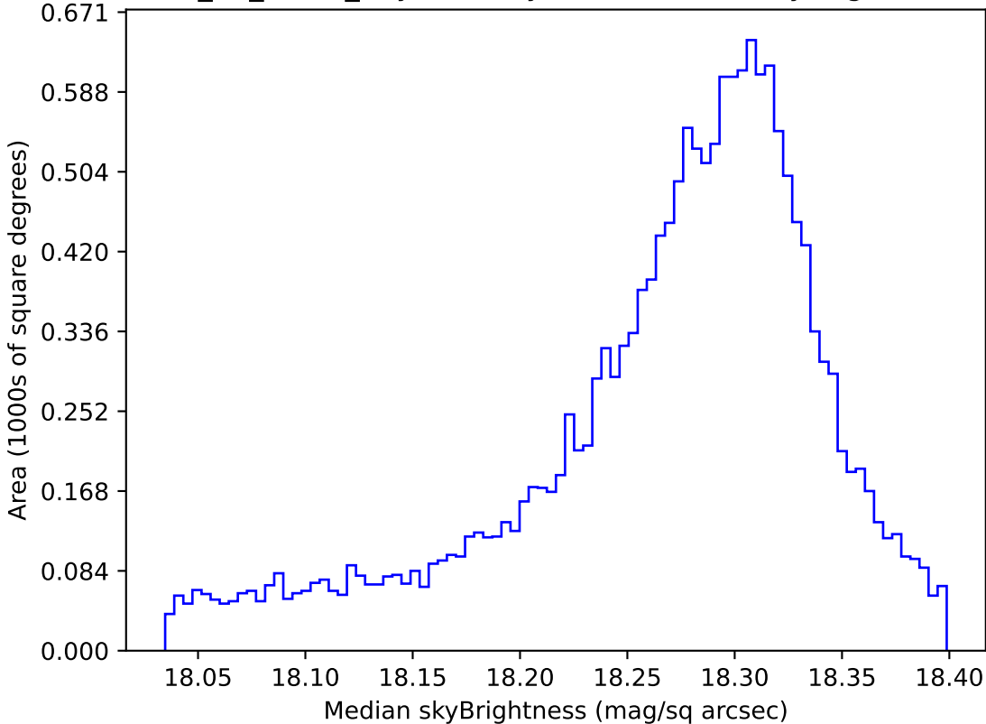
too_10_4v3.4_10yrs WFD y band: Median skyBrightness
