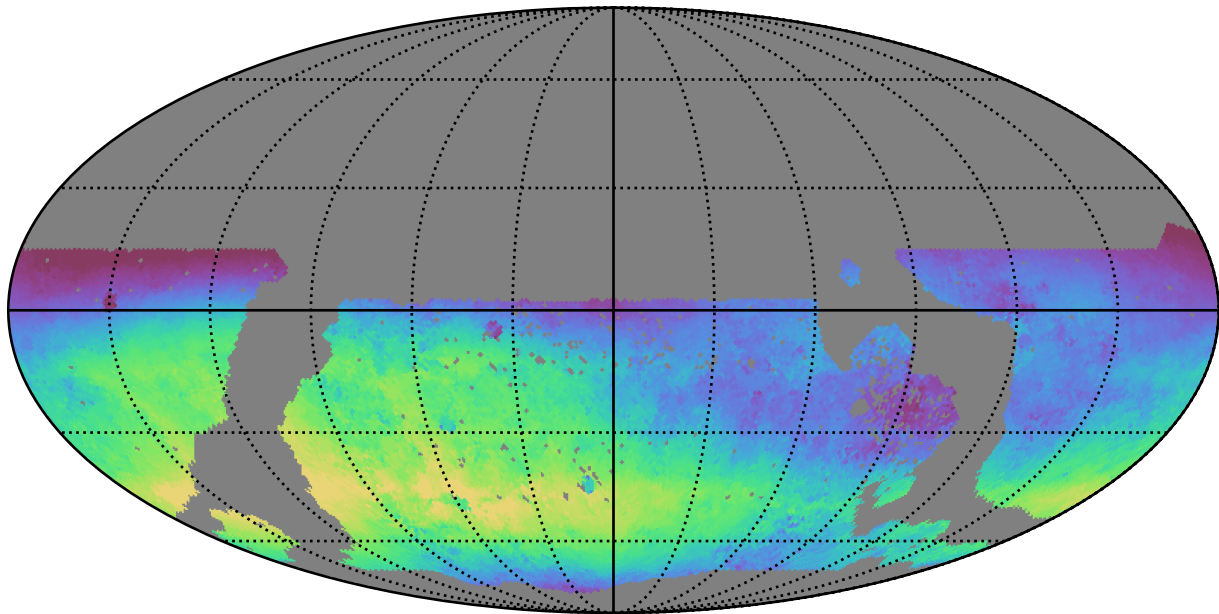
too_10_4v3.4_10yrs WFD u band: Median skyBrightness
