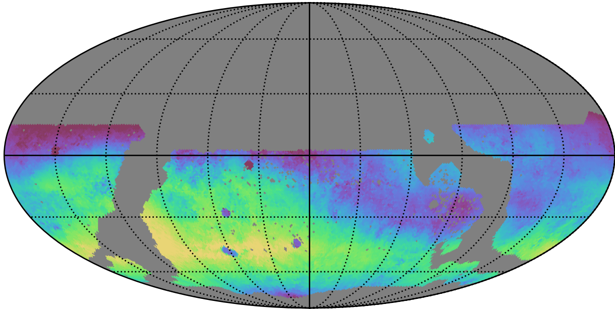
too_10_4v3.4_10yrs WFD r band: Median skyBrightness
