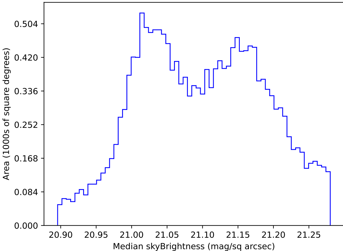
too_10_4v3.4_10yrs WFD r band: Median skyBrightness
