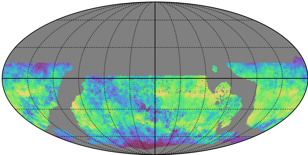
too_10_4v3.4_10yrs WFD i band: Median skyBrightness
