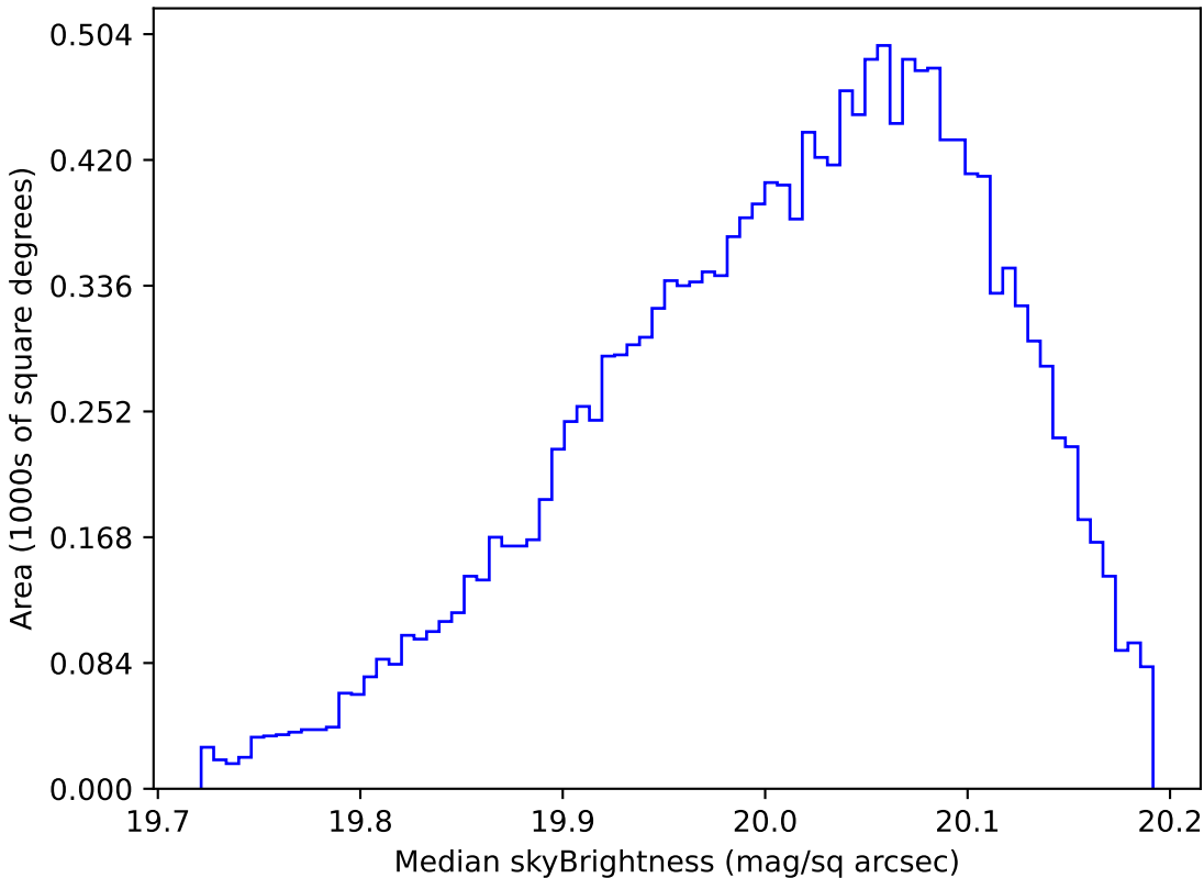
too_10_4v3.4_10yrs WFD i band: Median skyBrightness
