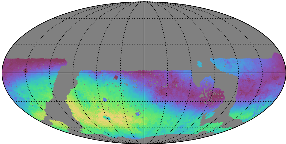
too_10_4v3.4_10yrs WFD g band: Median skyBrightness
