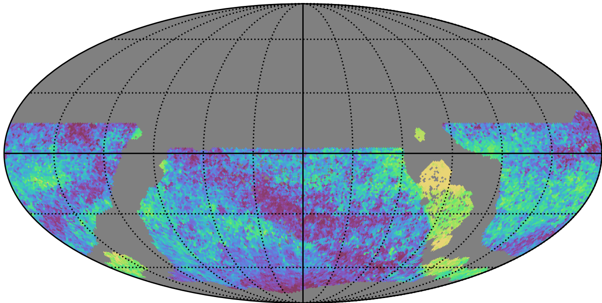
too_10_4v3.4_10yrs WFD all bands: Median skyBrightness
