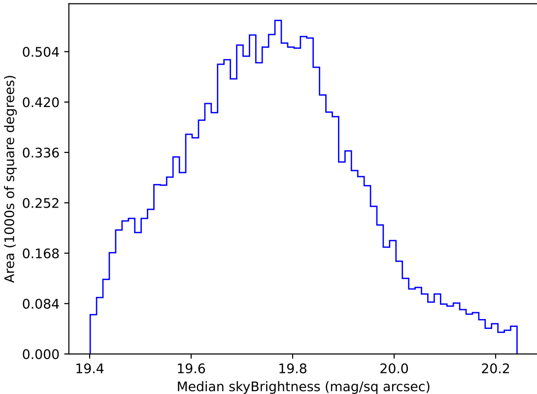
too_10_4v3.4_10yrs WFD all bands: Median skyBrightness
