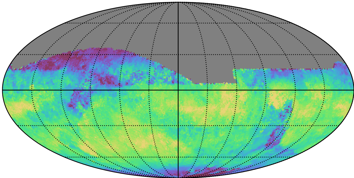
too_10_4v3.4_10yrs All sky z band: Median skyBrightness
