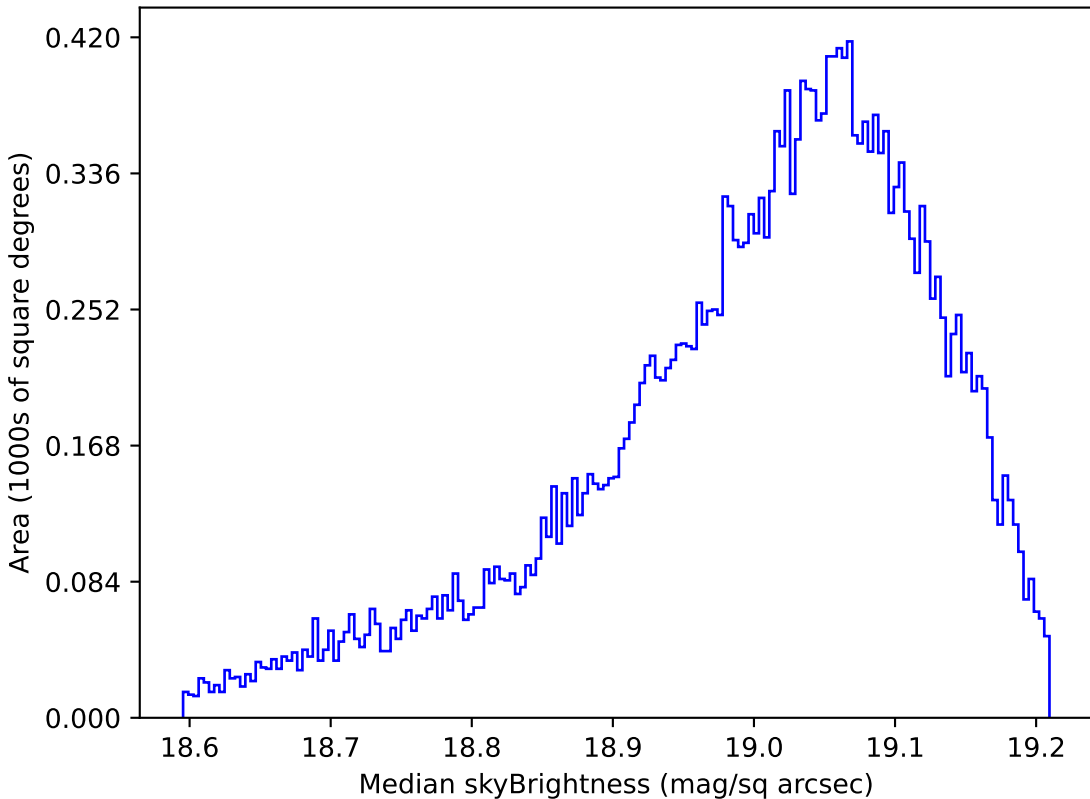
too_10_4v3.4_10yrs All sky z band: Median skyBrightness
