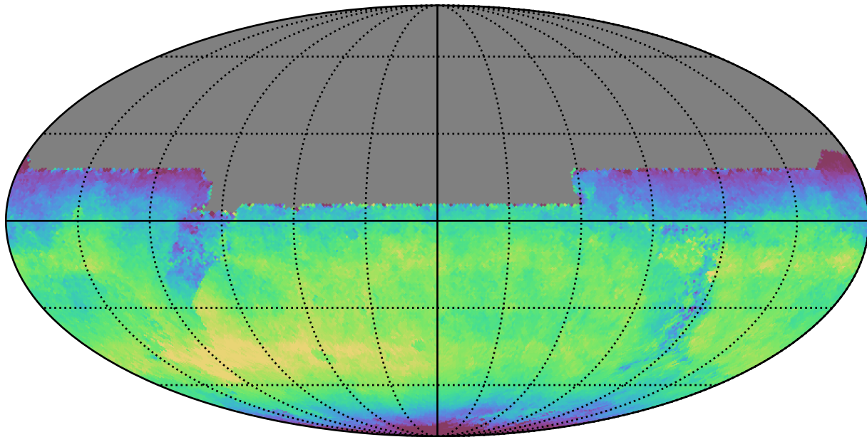
too_10_4v3.4_10yrs All sky y band: Median skyBrightness
