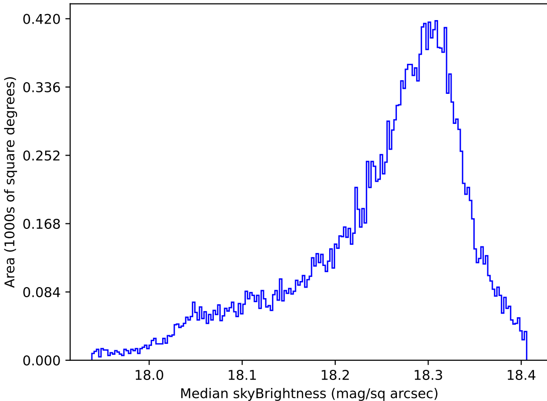
too_10_4v3.4_10yrs All sky y band: Median skyBrightness
