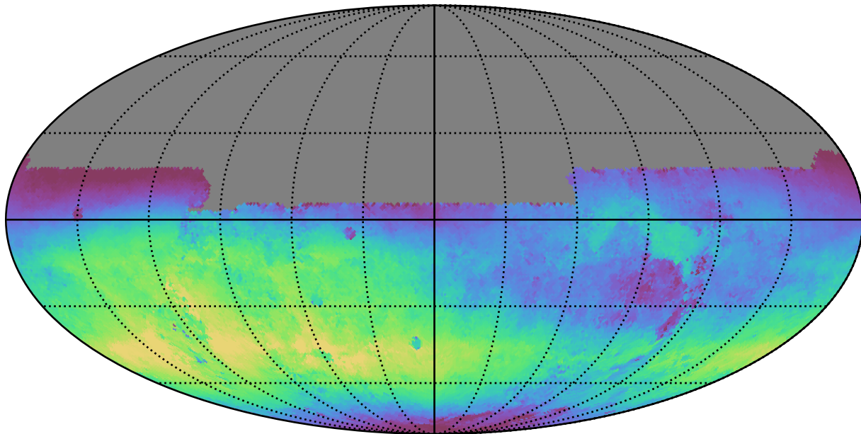
too_10_4v3.4_10yrs All sky u band: Median skyBrightness
