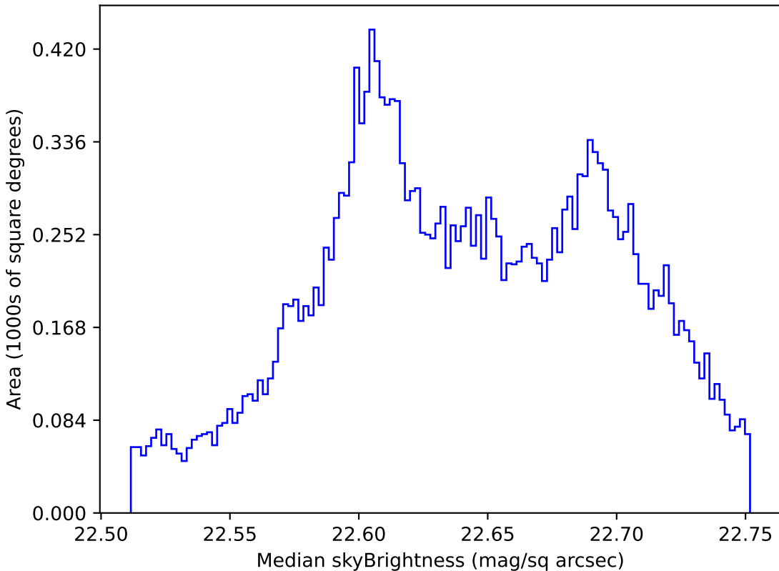
too_10_4v3.4_10yrs All sky u band: Median skyBrightness
