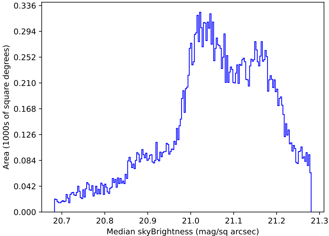
too_10_4v3.4_10yrs All sky r band: Median skyBrightness
