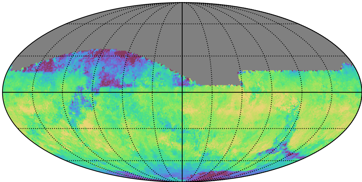
too_10_4v3.4_10yrs All sky i band: Median skyBrightness
