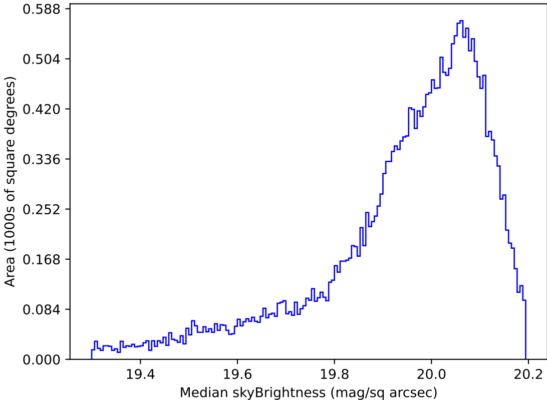
too_10_4v3.4_10yrs All sky i band: Median skyBrightness
