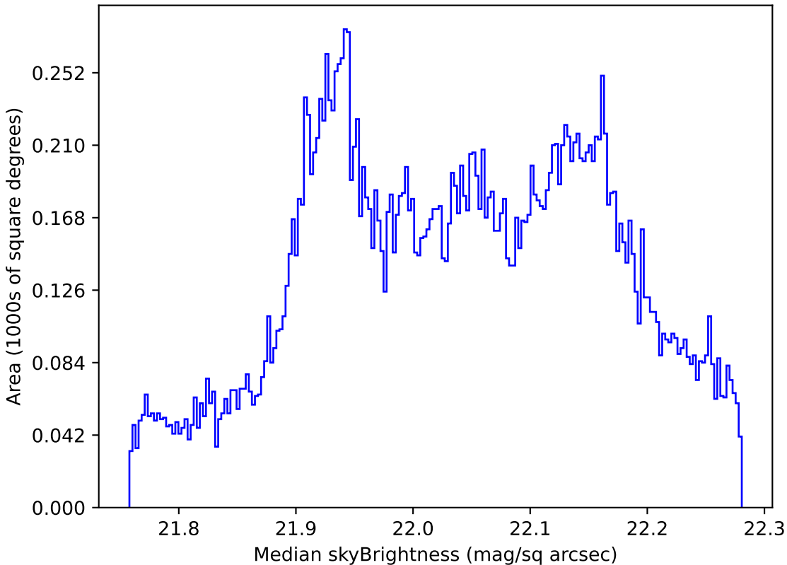
too_10_4v3.4_10yrs All sky g band: Median skyBrightness
