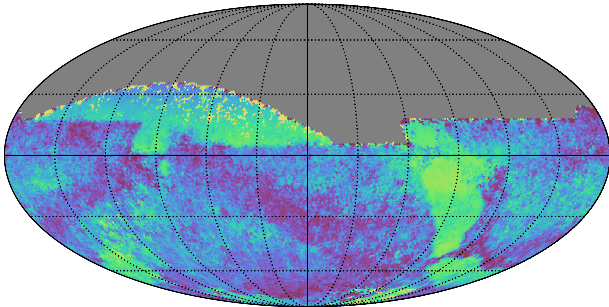
too_10_4v3.4_10yrs All sky all bands: Median skyBrightness
