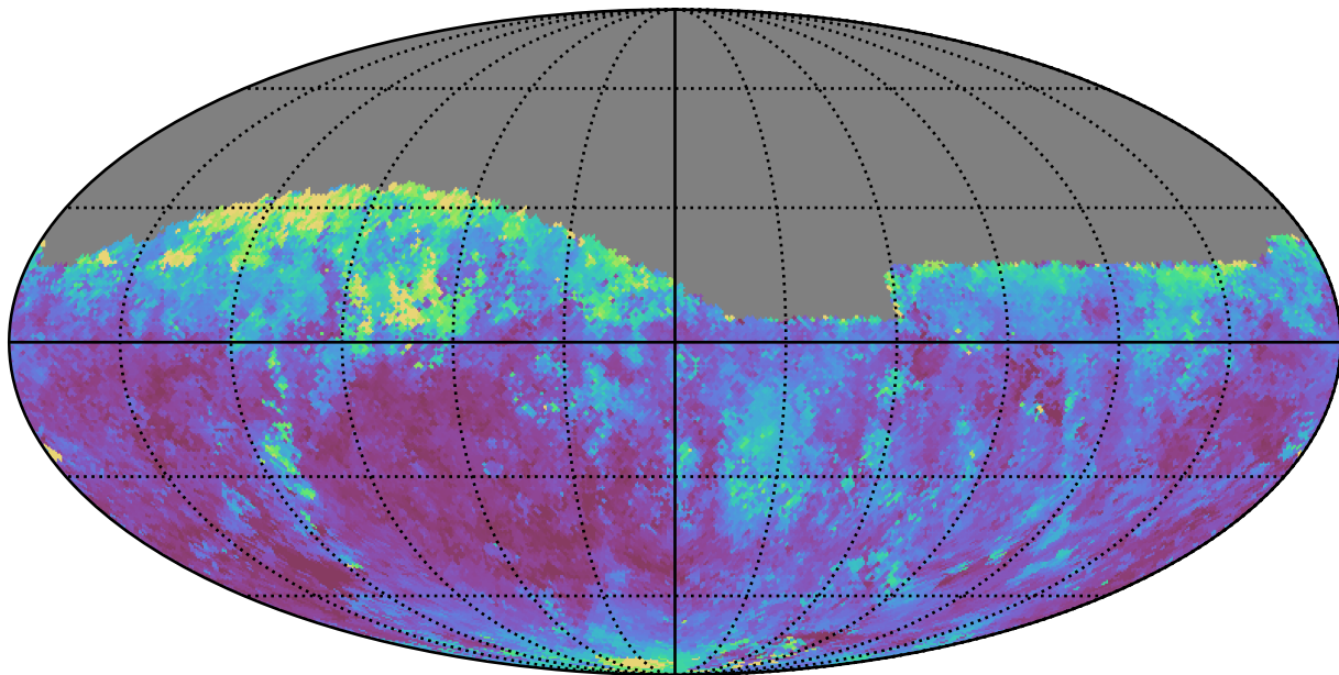
too_10_4v3.4_10yrs Yr 1 z band: Median seeingGeom
