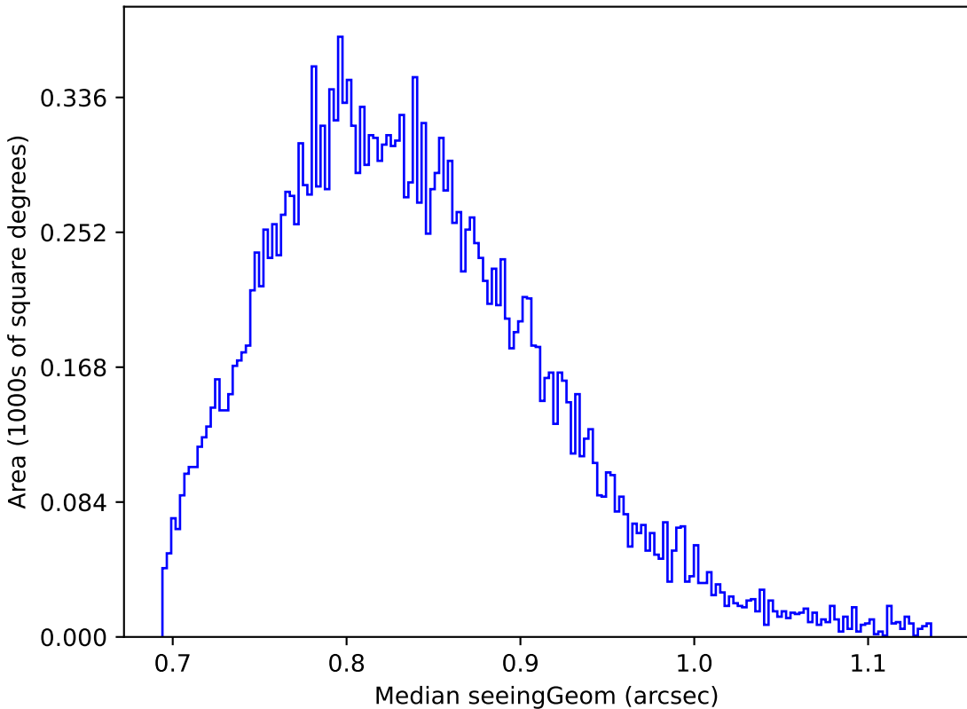
too_10_4v3.4_10yrs Yr 1 y band: Median seeingGeom
