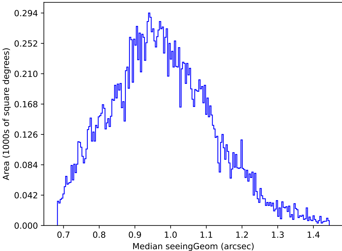
too_10_4v3.4_10yrs Yr 1 u band: Median seeingGeom
