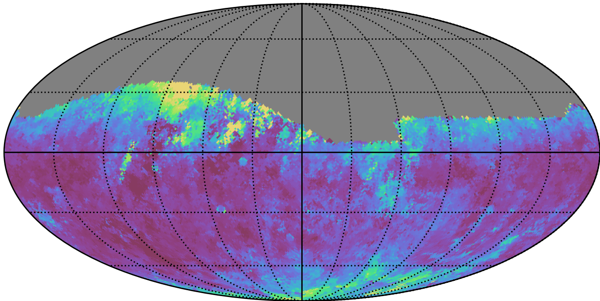
too_10_4v3.4_10yrs Yr 1 r band: Median seeingGeom
