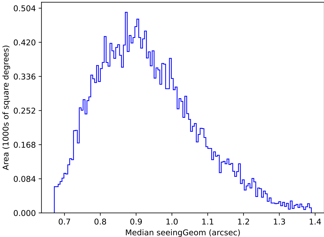
too_10_4v3.4_10yrs Yr 1 g band: Median seeingGeom
