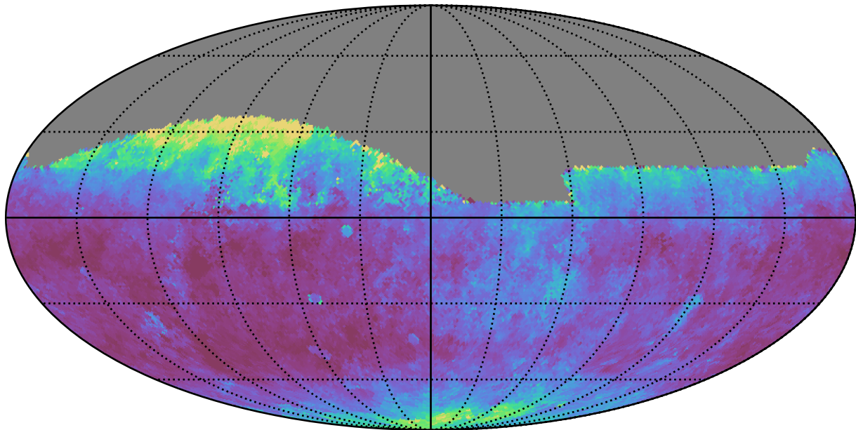
too_10_4v3.4_10yrs Yr 1 all bands: Median seeingGeom
